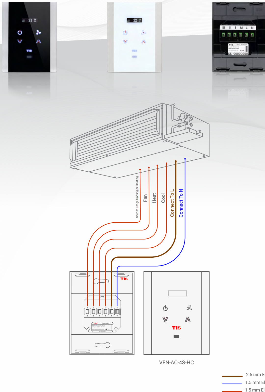
Figure 1: VEN-AC-4S-HC & FCU Connection Diagram
