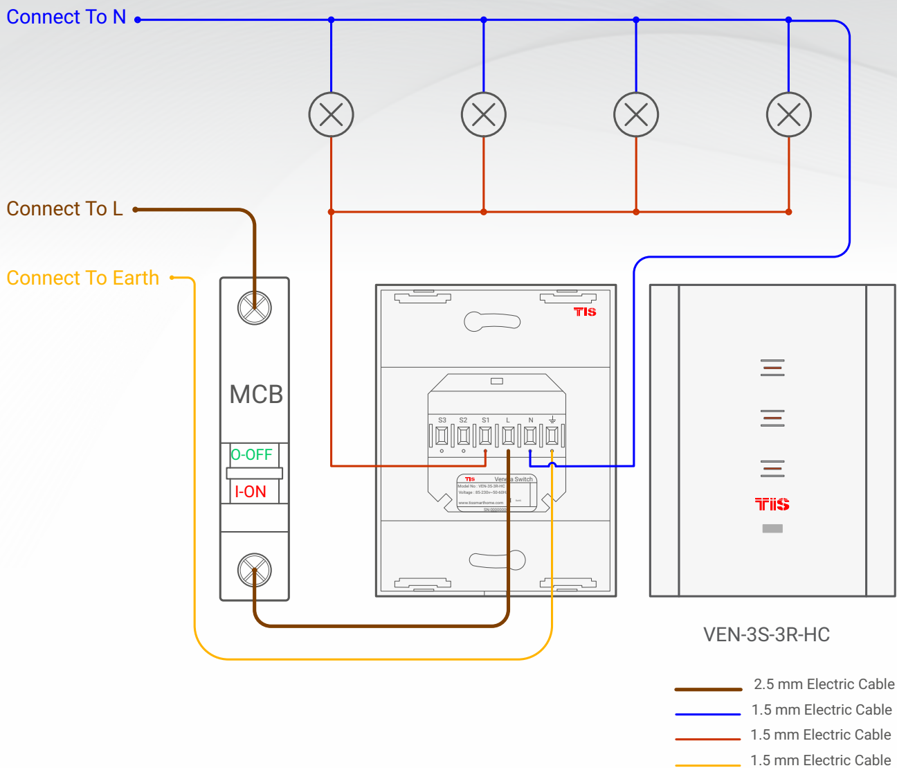
▲ Figure 1: VEN-3S-3R-HC Lights Connection Diagram
