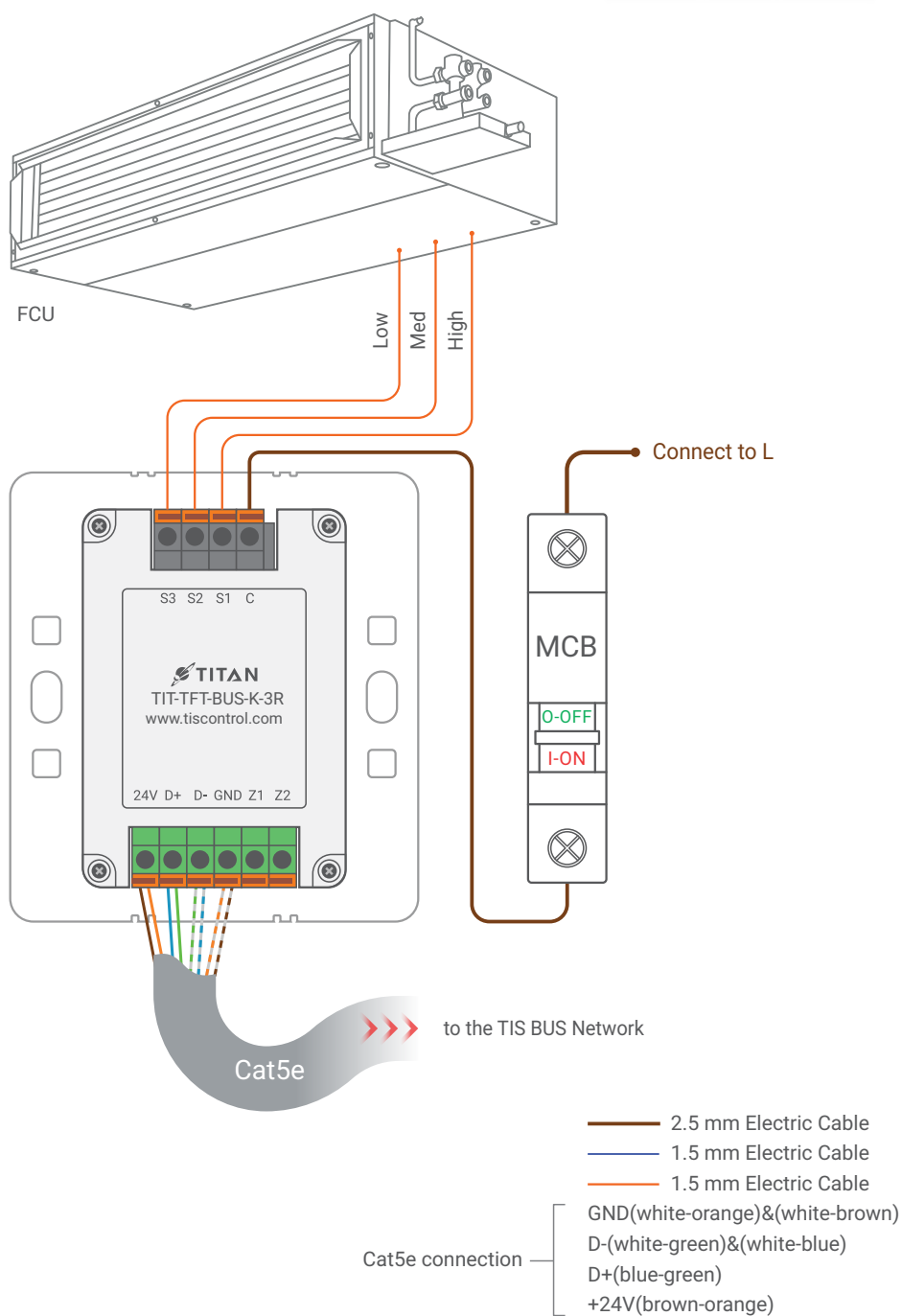
▲ Figure 2: TIT-TFT-BUS-K-3R & FCU Connection Diagram
