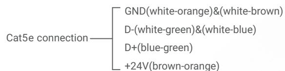
▲ Figure 8: TIT-TFT-BUS-K-3R Module's Bus Connection Color Coding
