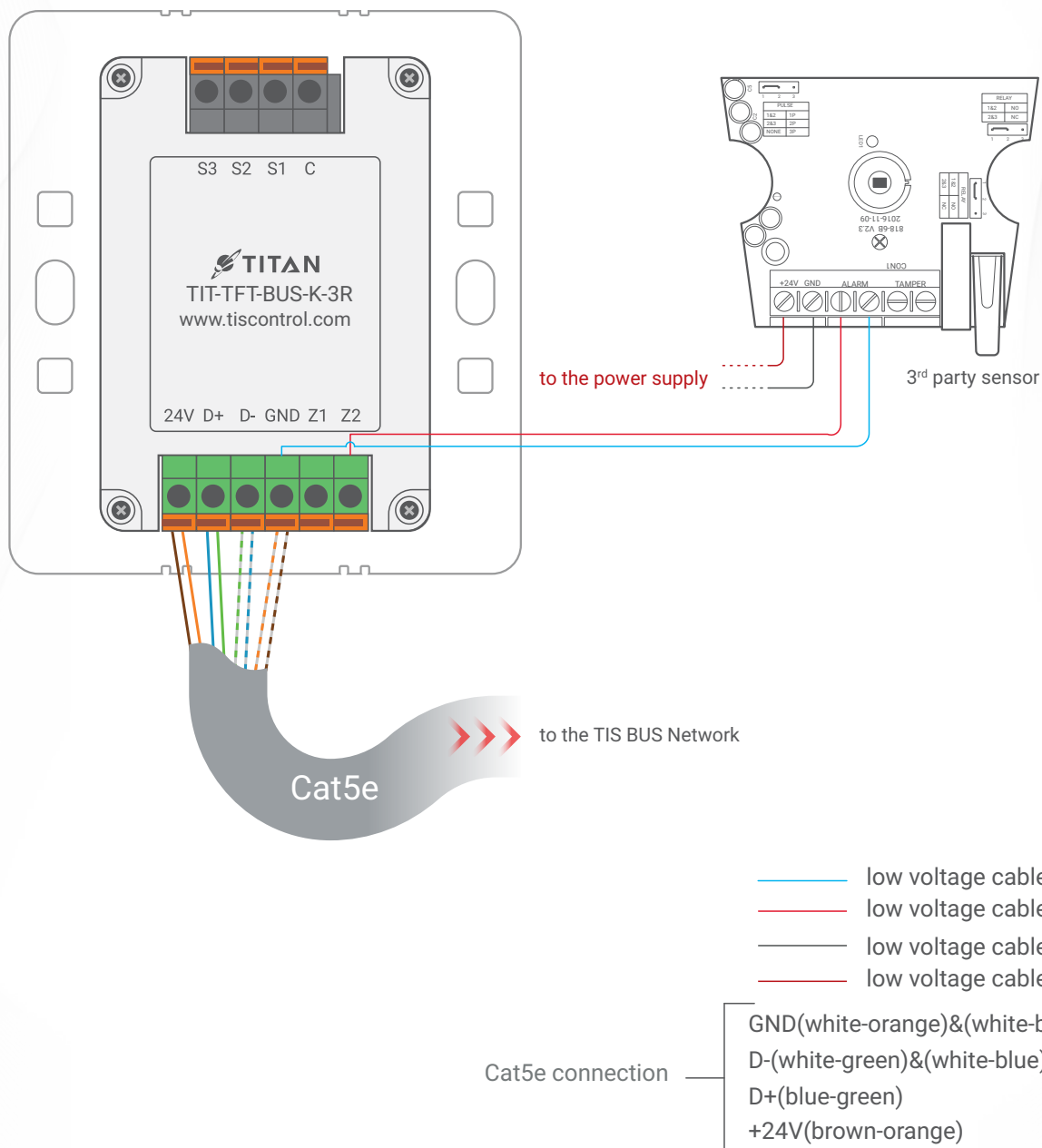
▲ Figure 7: TIT-TFT-BUS-K-3R & 3rd Party Sensor Connection Diagram
