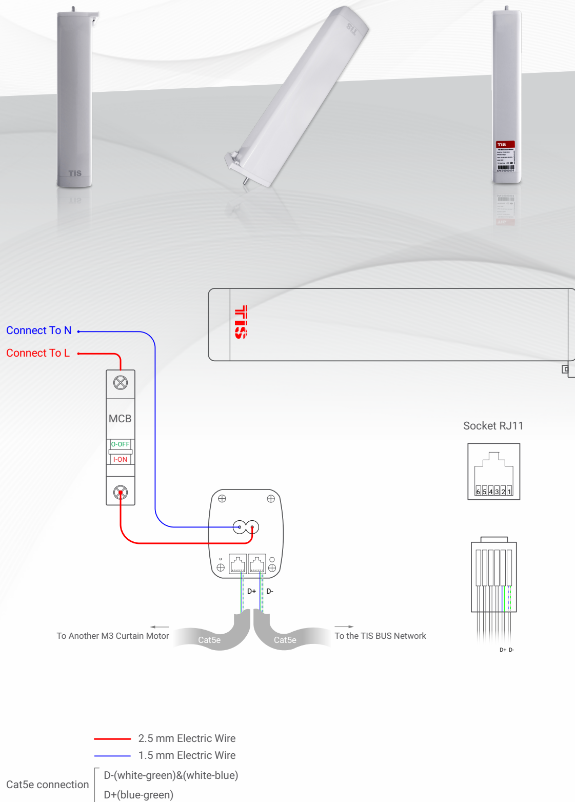
▲ Figure 1: Curtain Motor Configuration Diagram
