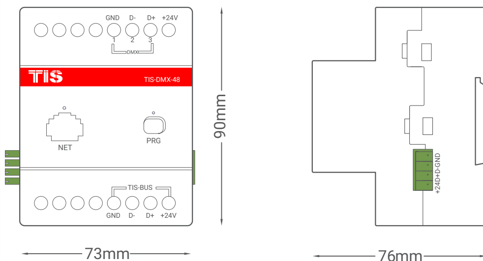
▲ Figure 6: TIS-DMX-48 Module's Dimensions
