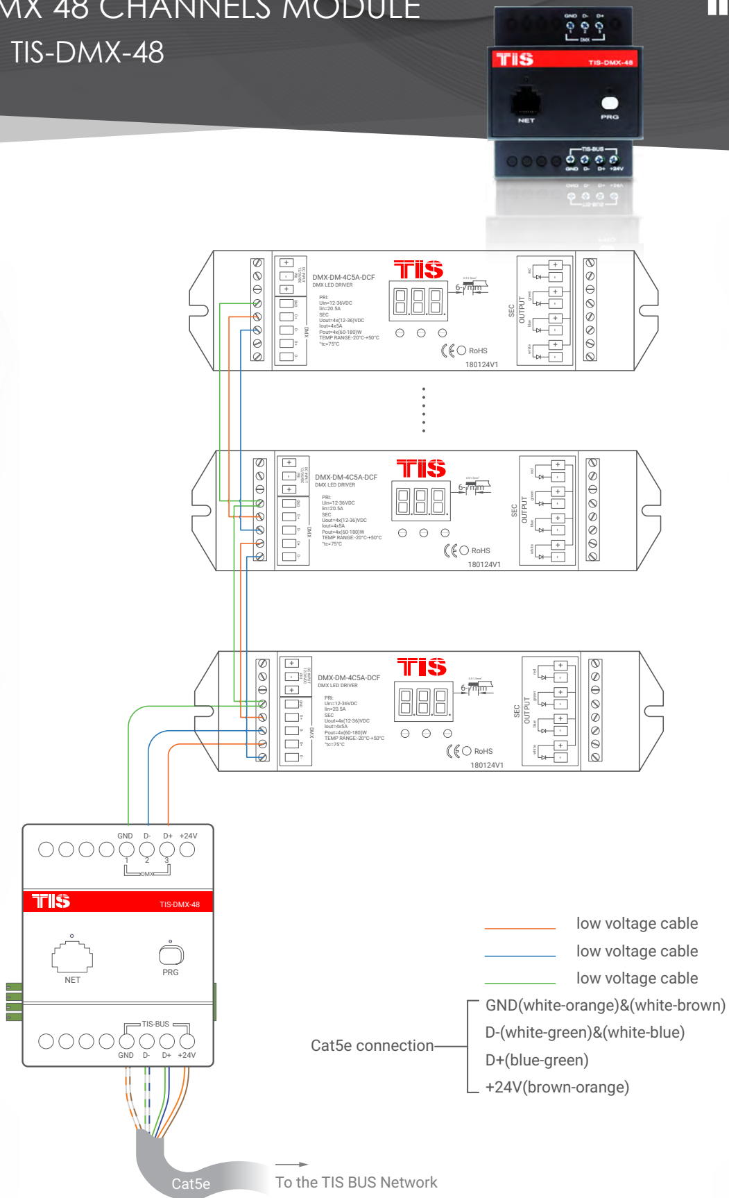
▲ Figure 3: DMX & DMX Driver's Connection Diagram
