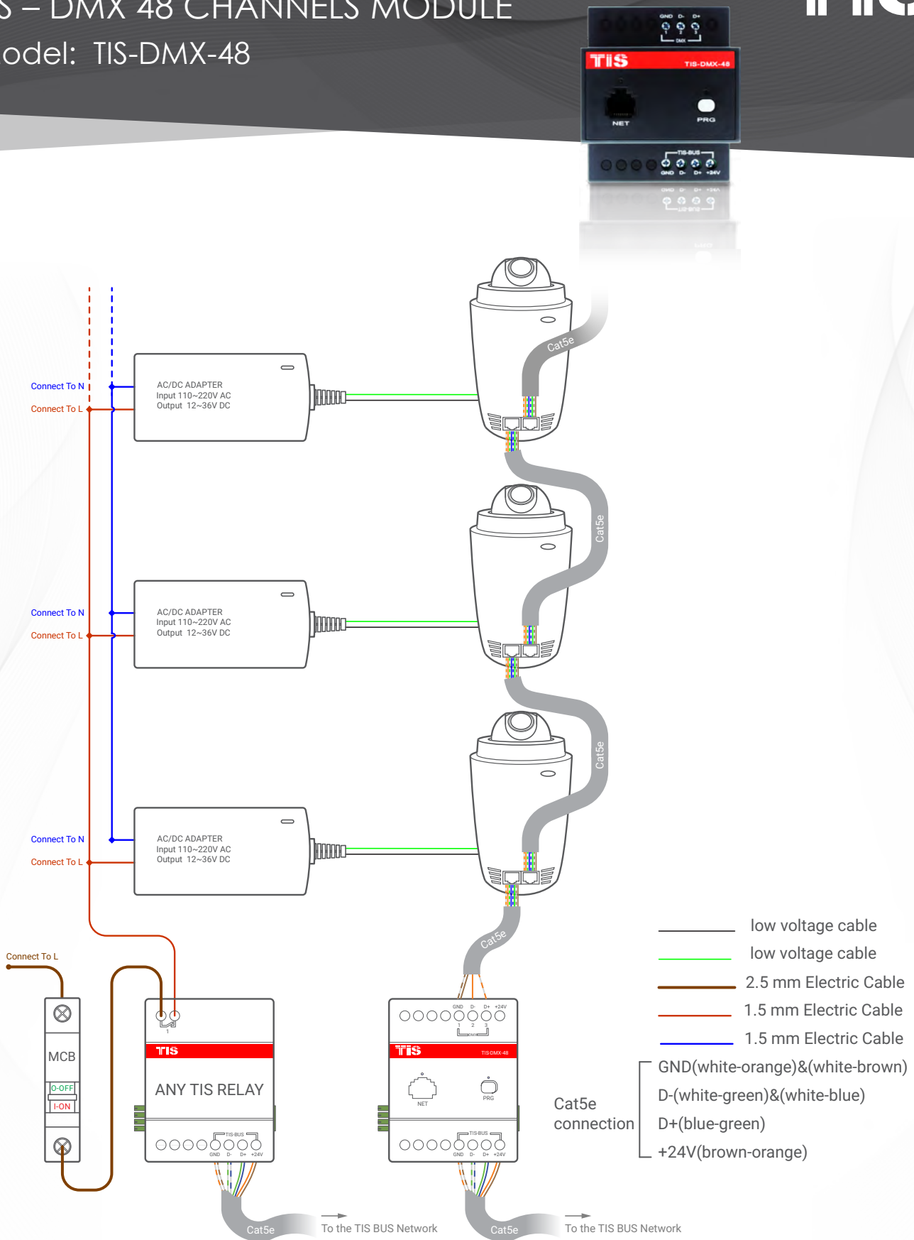
▲ Figure 2: DMX Lights Connection Diagram
