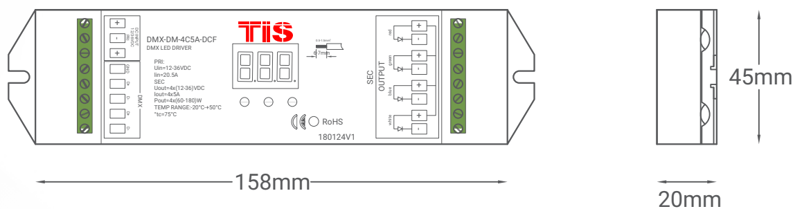
▲ Figure 7: DMX Driver's Dimensions
