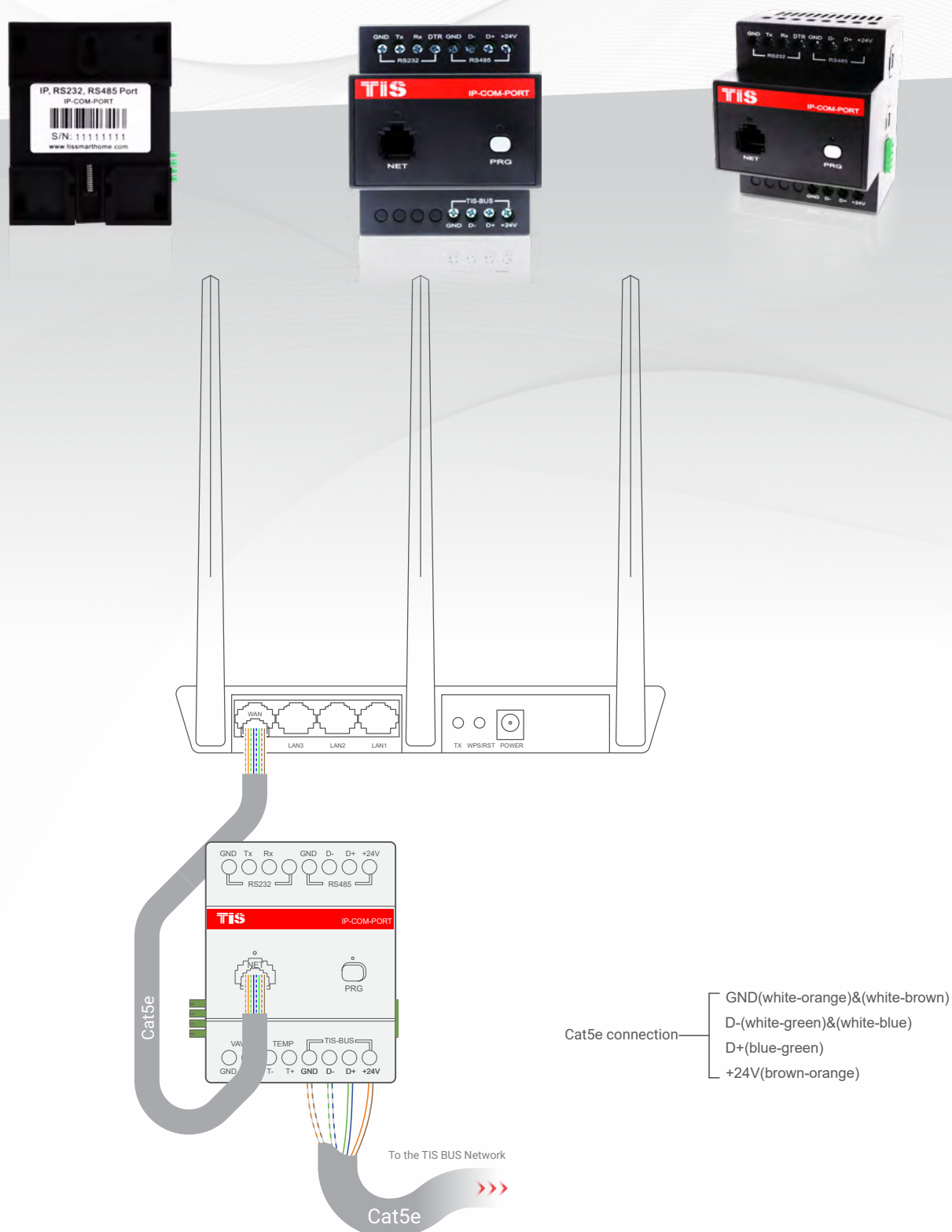
Figure 1: Ethernet Router Connection Diagram
