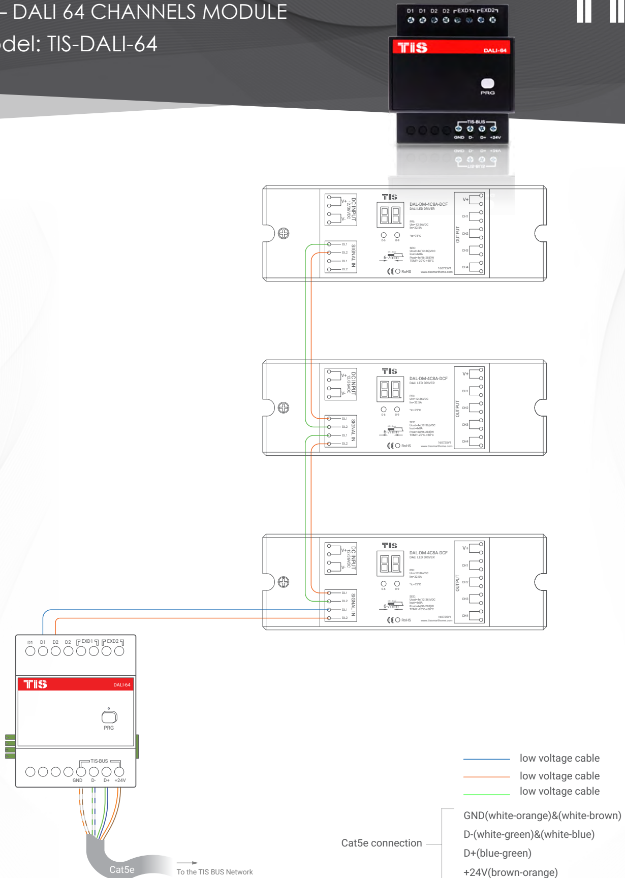
▲ Figure 3: DALI & DALI Driver Connection Diagram
