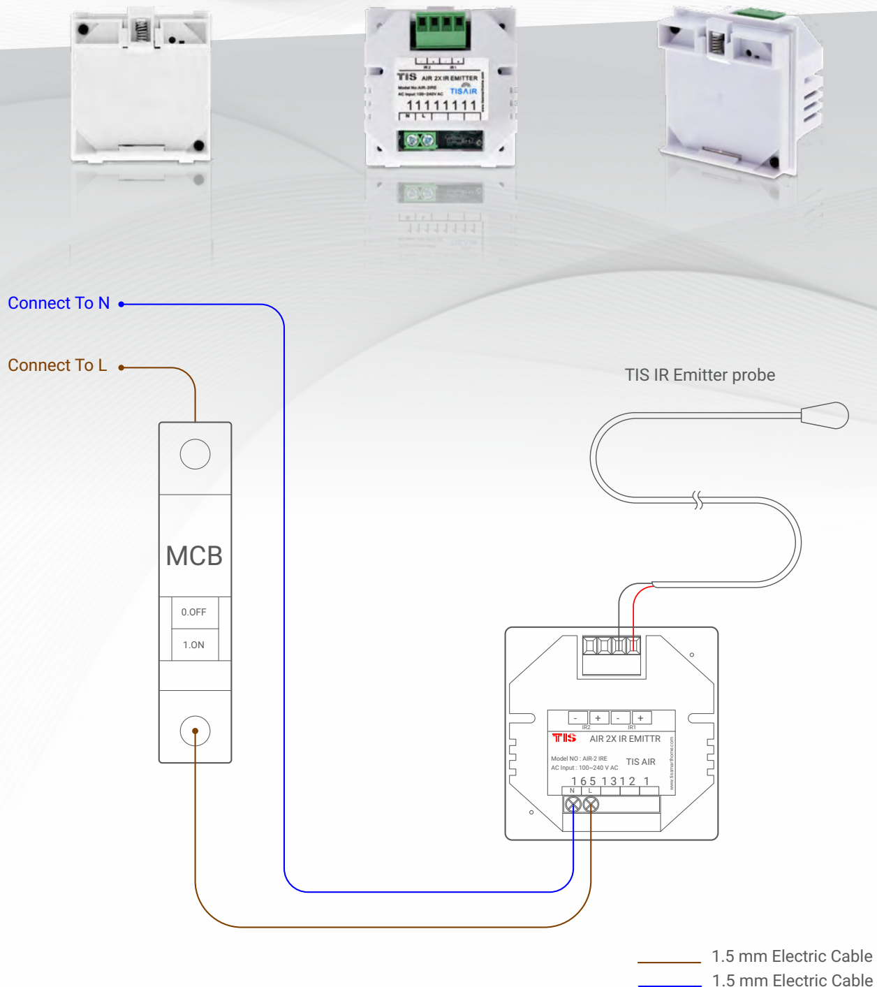
▲ Figure 1: LED Dimmer Connection Diagram
